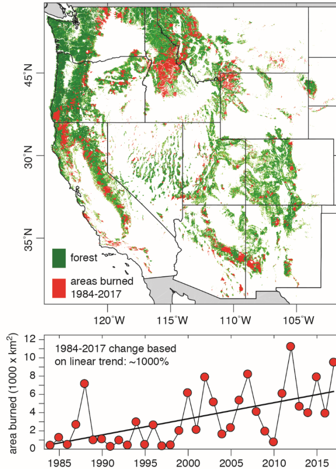
Fig. 3. Western U.S. forest fire area for 1984 to 2017. (Top) Map of forest fire areas. (Bottom) Annual forest fire area based on the U.S. Forest Service Monitoring Trends in Burn Severity (MTBS) project for 1984 to 2016 (90) and the MODIS version 6 burned area product for 2017 (91). The MODIS burned-area record was linearly calibrated to the MTBS record during overlapping years of 2001 to 2016. The linear trend is based on least-squares regression.
